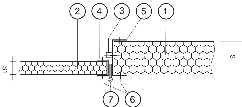
SCALE 1:5
