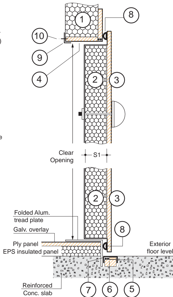
A - A CROSS SECTION SCALE 1:10
