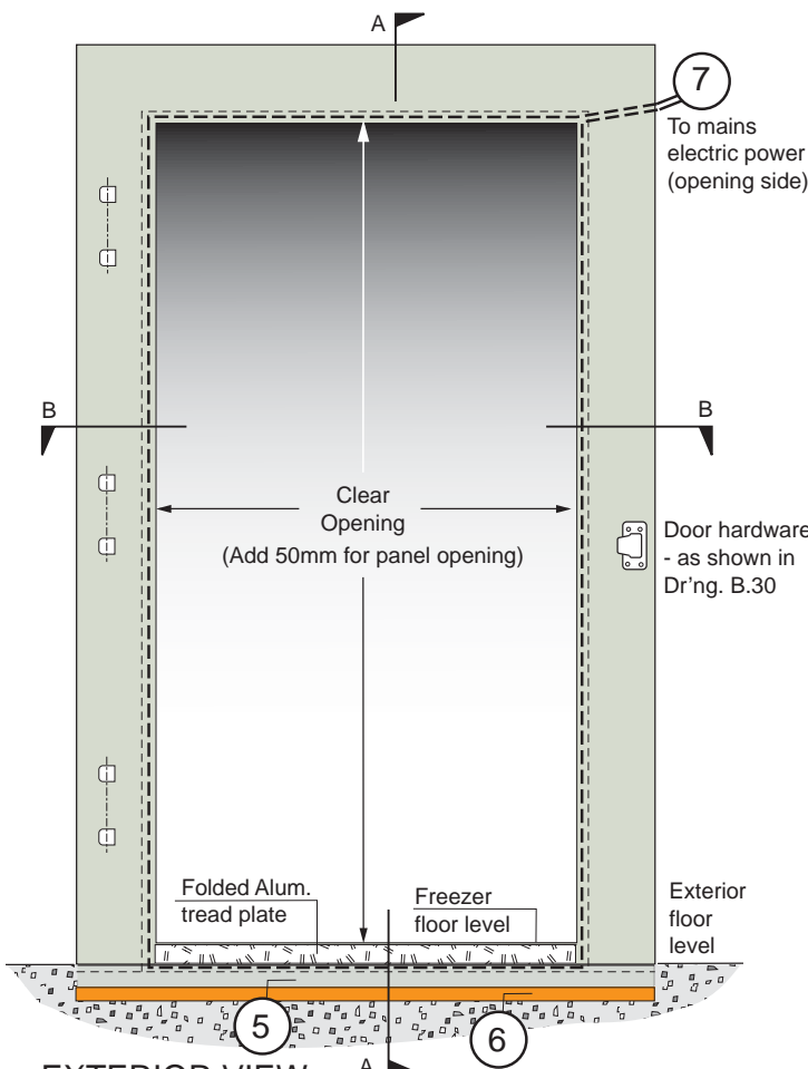
EXTERIOR VIEW SCALE 1:20
