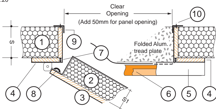
EXTERIOR VIEW SCALE 1:20
